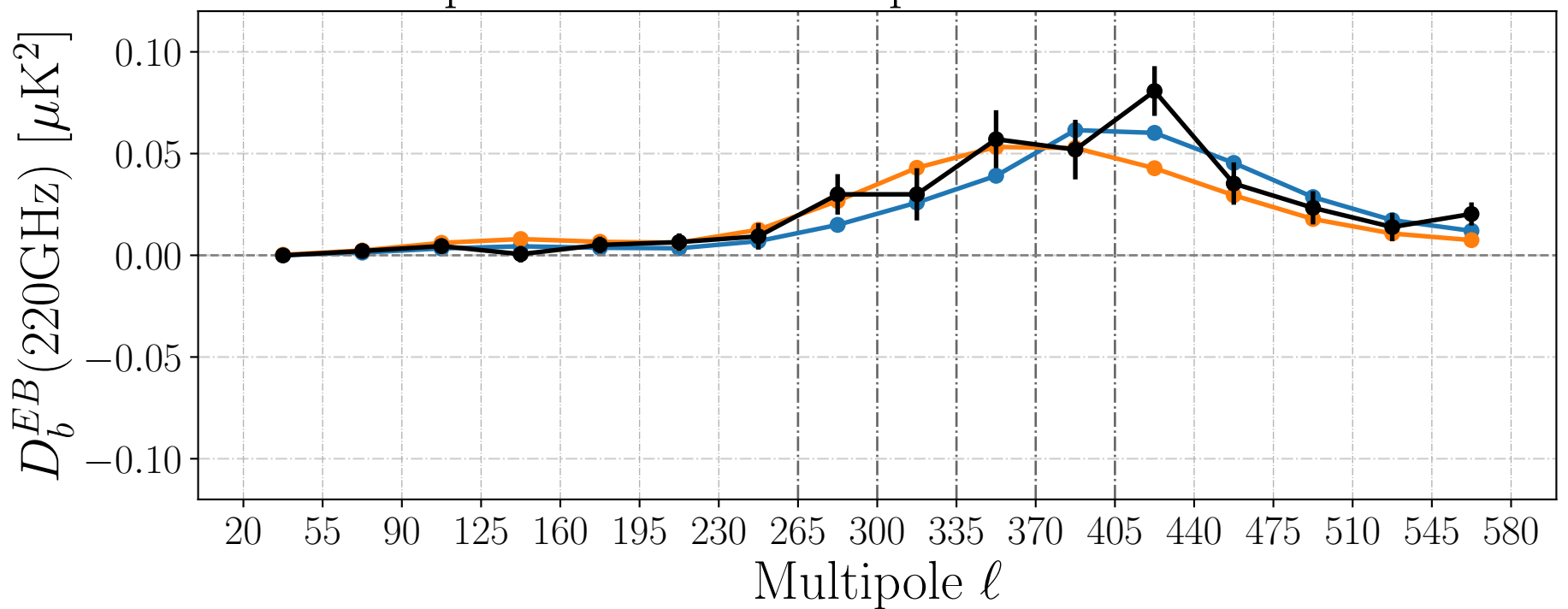
EB Spectrum After Bandpower Window Function
