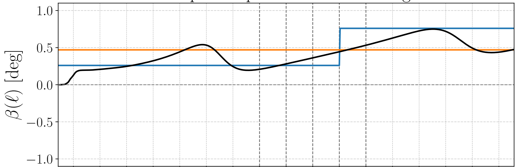
Multipole Dependent Rotation Angle
