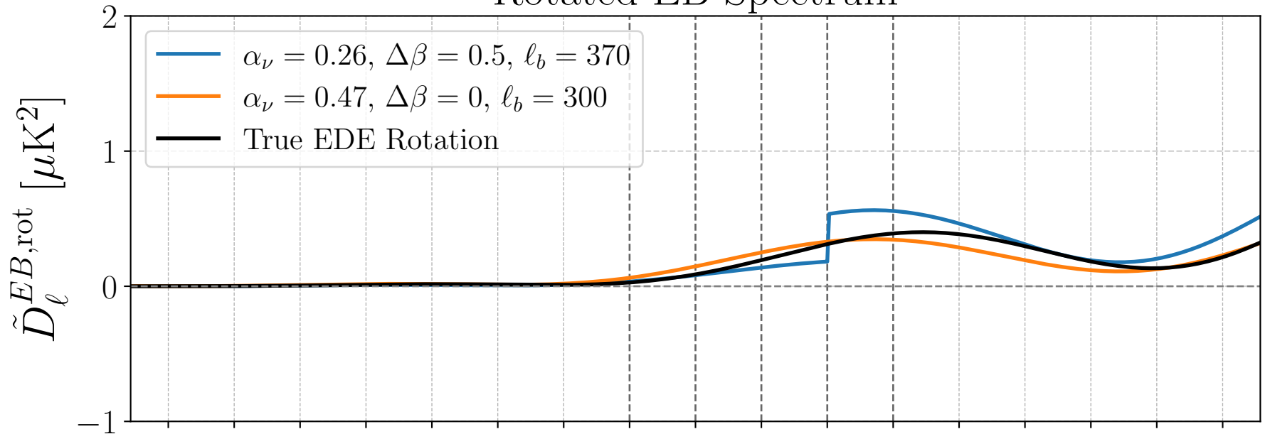
Rotated EB Spectrum
