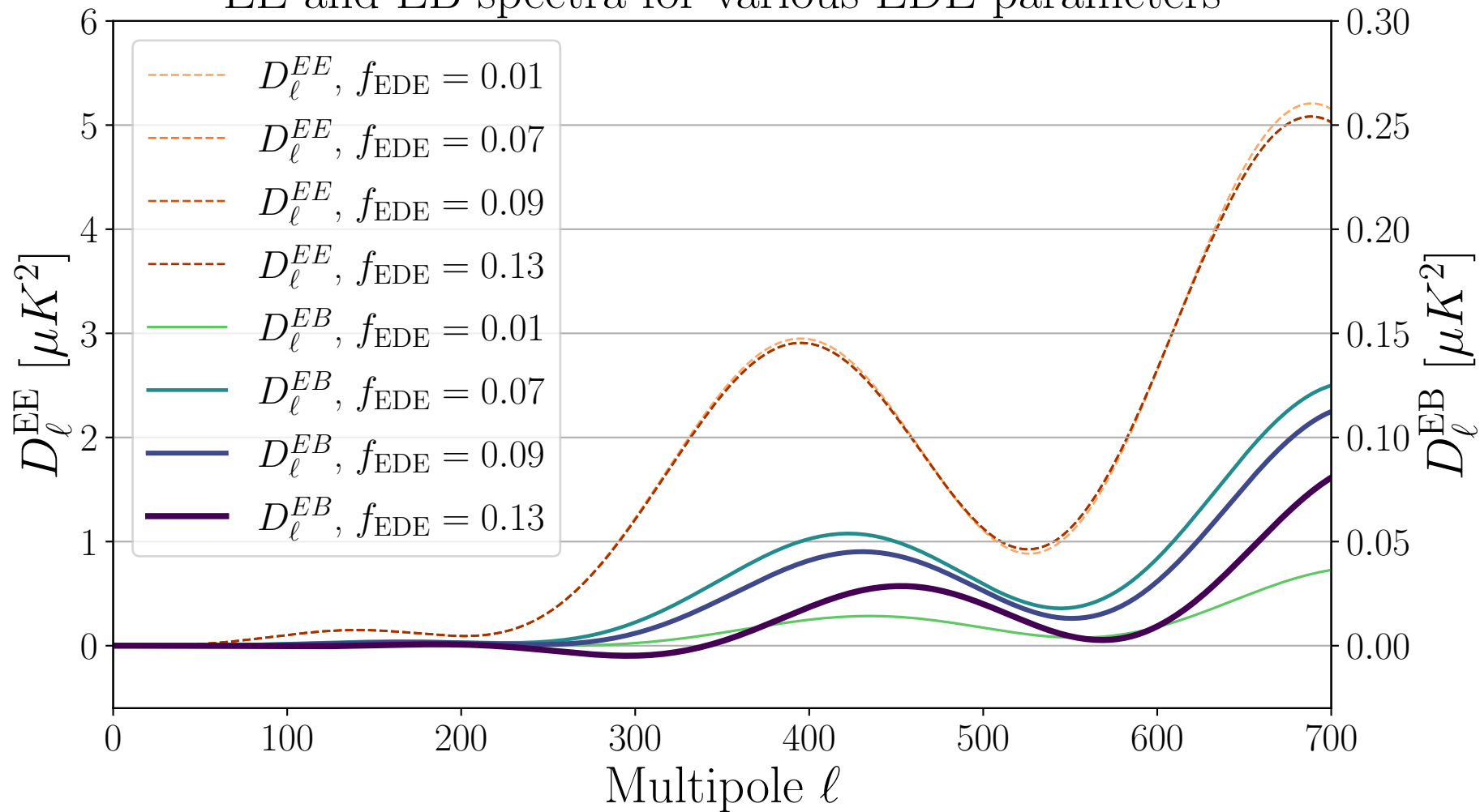
EE and EB spectra for various EDE parameters
