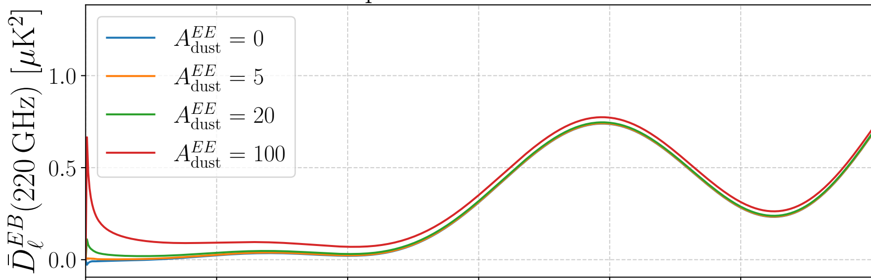
EB Spectrum Before BPWF
