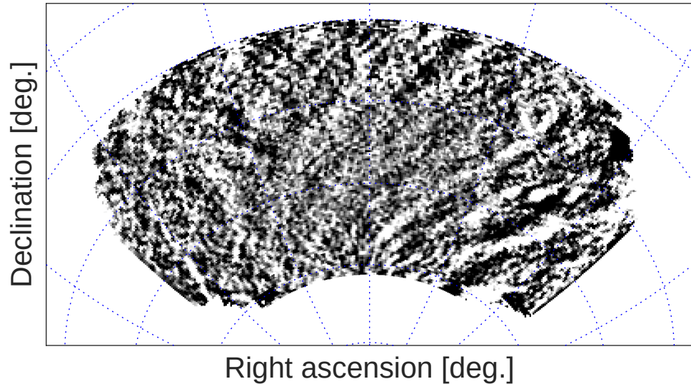
dust U signal at 95 GHz
