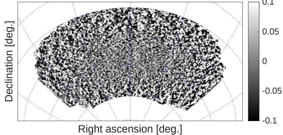
dust U noise at 95 GHz simulation realization
