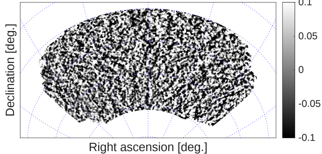
scaled 353 GHz U noise simulation realization
