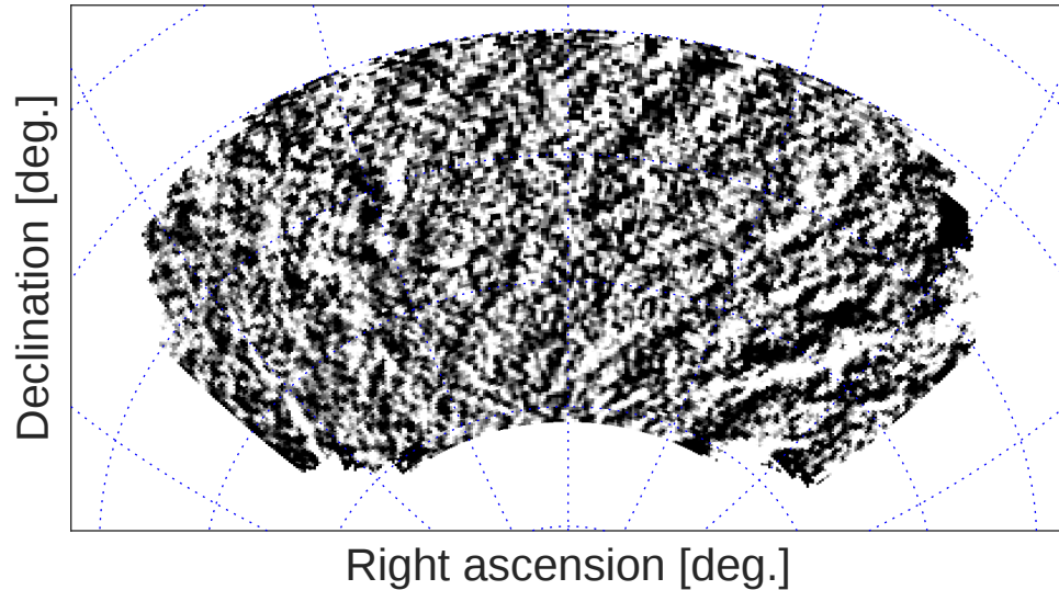
scaled 353 GHz U signal
