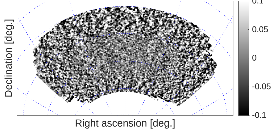
dust Q noise at 95 GHz simulation realization
