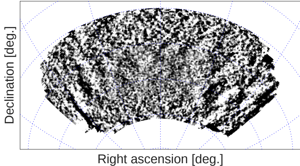
dust Q signal at 95 GHz
