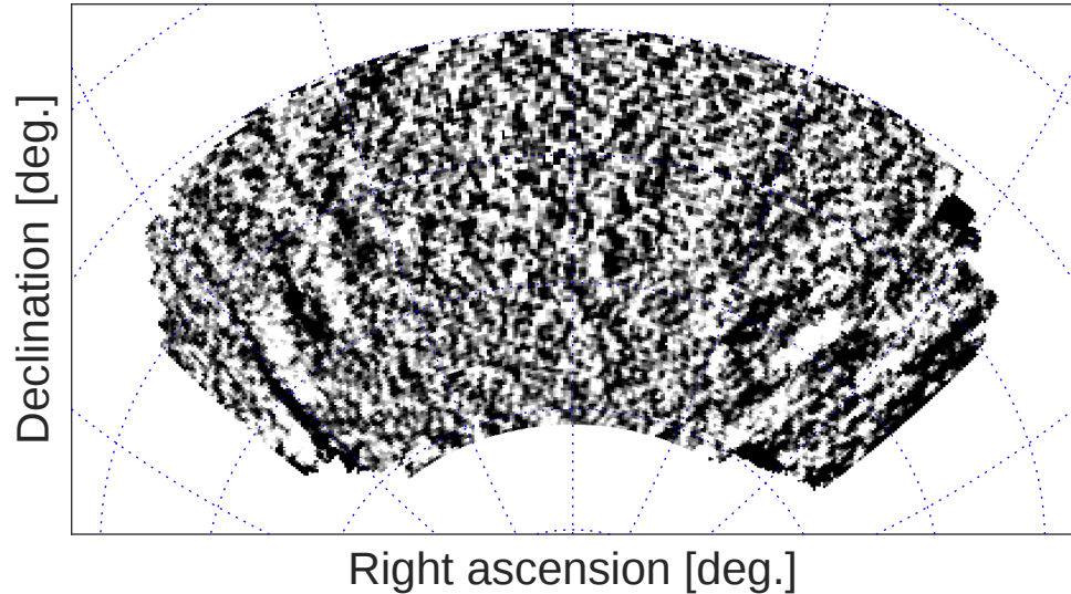
scaled 353 GHz Q signal
