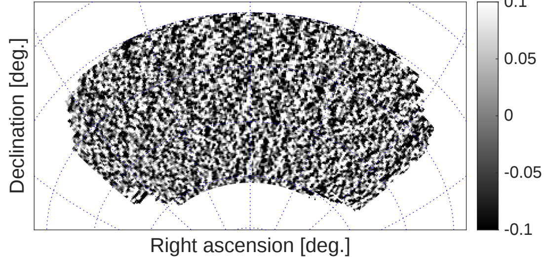
scaled 353 GHz Q noise simulation realization
