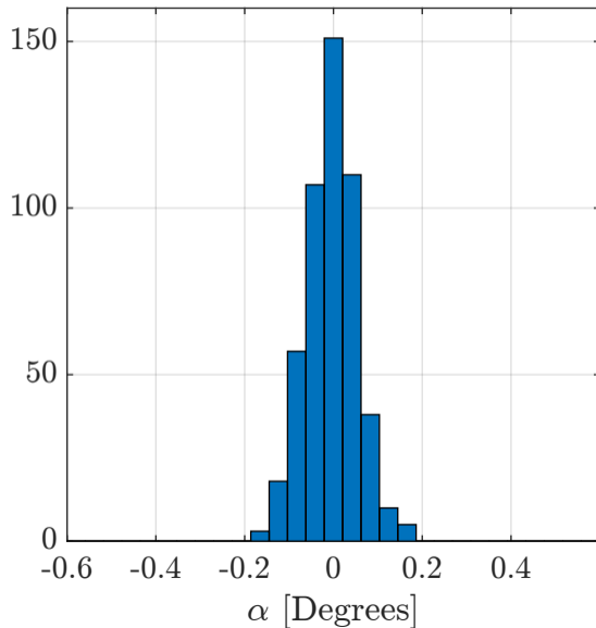
Fit over bins 2 through 15 EB: \langle \alpha \rangle = -0.00 \mid \sigma_\alpha = 0.06
