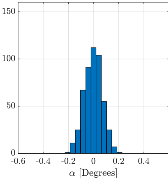
Fit over bins 11 through 15 EB: \langle \alpha \rangle = -0.00 \mid \sigma_\alpha = 0.07
