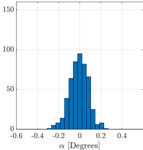
Fit over bins 2 through 10 EB: \langle \alpha \rangle = -0.01 \mid \sigma_\alpha = 0.09
