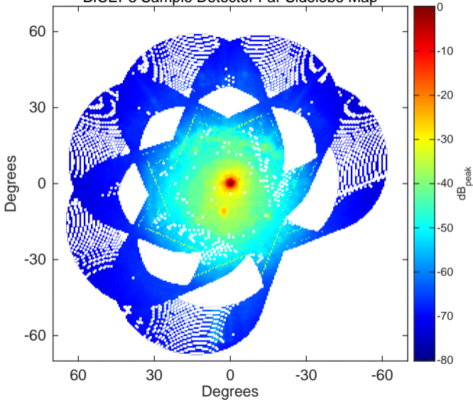
BICEP3 Sample Detector Far Sidelobe Map
