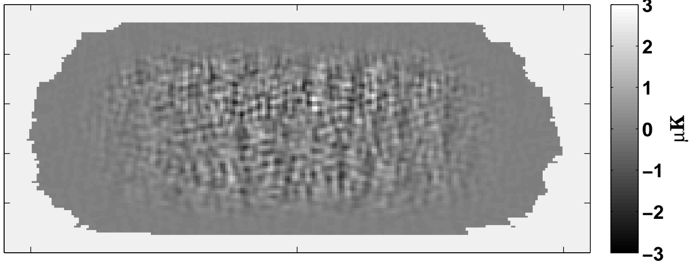
Observation Matrix
