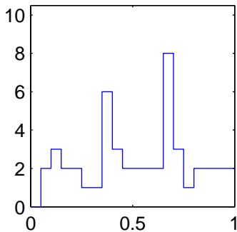
Band powers 1–9 \chi^2
