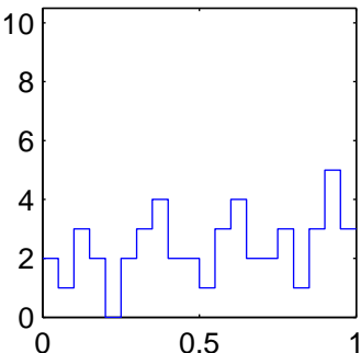
Band powers 1–5 \chi
