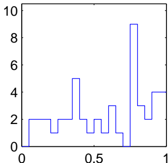
Band powers 1–9 \chi
