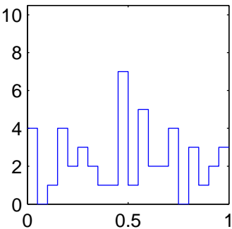
Band powers 1–5 \chi^2
