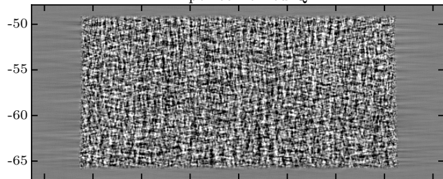
Deflection in RA
