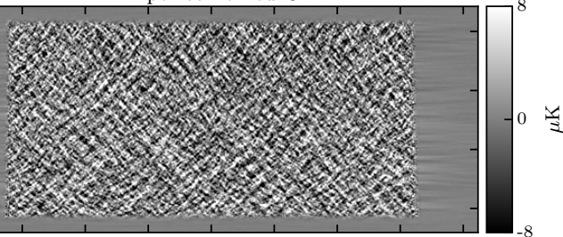
Deflection in Dec
