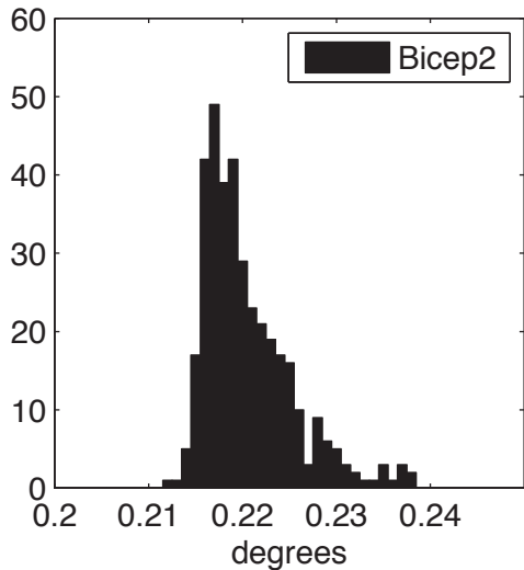
Bicep2 Beam Width
