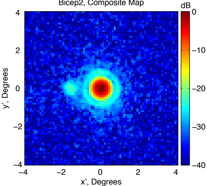
Bicep2, Composite Map
