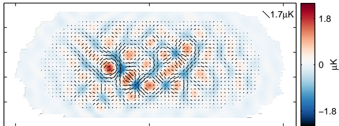
Simulation: B from lensed- \Lambda CDM+noise
