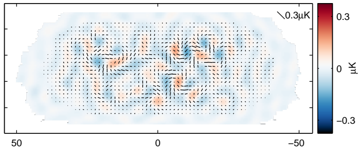
Simulation: B from lensed- \Lambda CDM+noise
